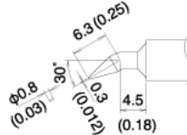
T22-JD08 SHAPE-0.8JD
