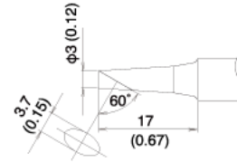
T22-C3 SHAPE-3C
