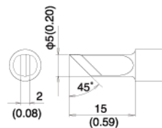
T22-K SHAPE-K
