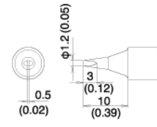
T22-D12 SHAPE-1.2D
