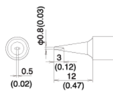
T22-D08 SHAPE-0.8D
