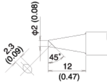
T22-BC2 SHAPE-2BC
